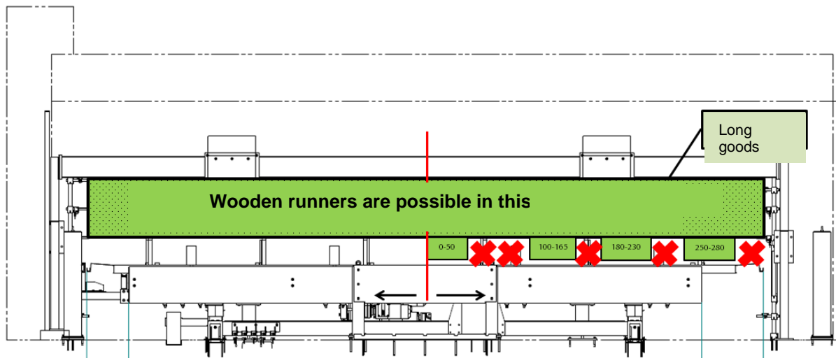
Figure 17: Attachment of wooden runners
