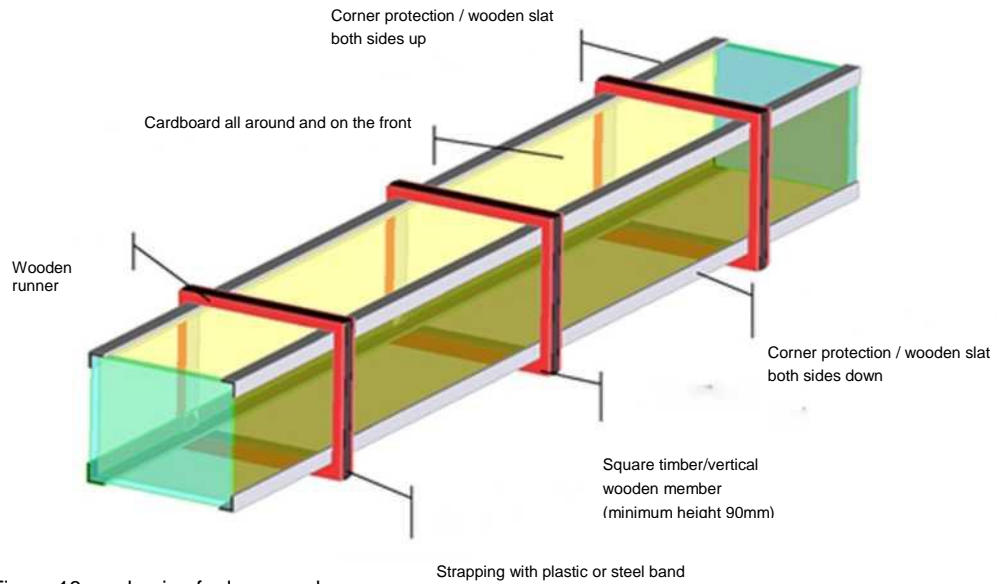
Figure 16: packaging for long goods
